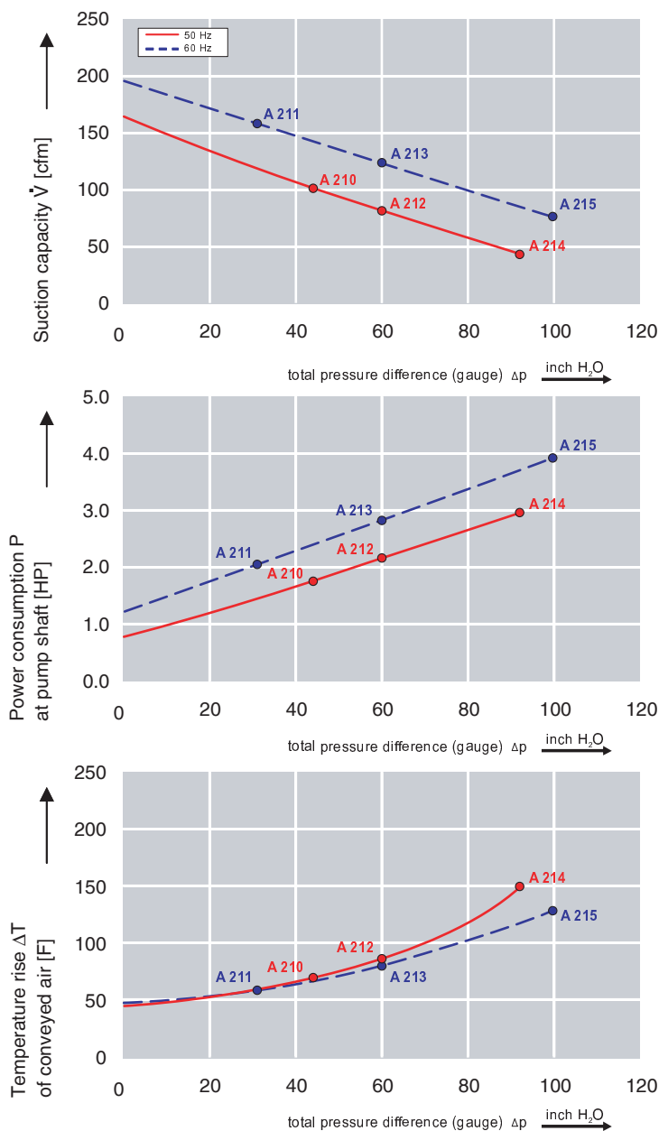
Performance curve for Compressor
