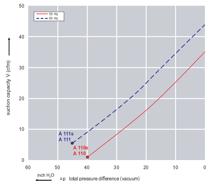
Performance curve for Vacuum pump
