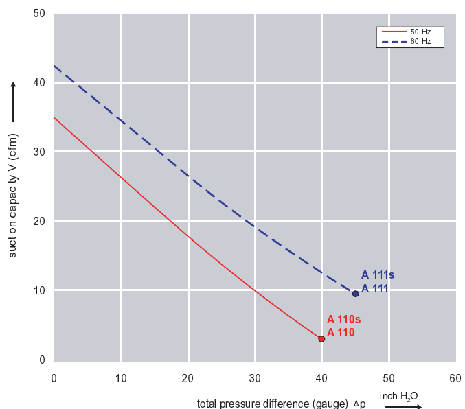
Performance curve for Compressor
